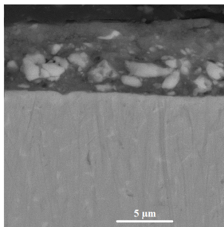
Figure 2. SEM image of cross-section of graded coating
