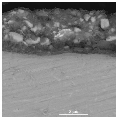
Figure 1. SEM image of cross-section of compoaite coating
